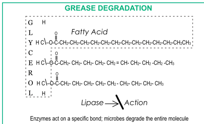
Figure 1: Typically, grease molecules are comprised of 3 fatty acids, varying in length, and attached to a glycerol backbone. A variety of microbes have the ability to generate enzymes that breakdown the fatty acids found in glycerol. However, these microbes aren't able to generate the enzymes that degrade the fatty acids. GeoKleen TM 's fatty acid degrading microbial strain does produce the enzymes necessary for the complete breakdown of fatty acids.
