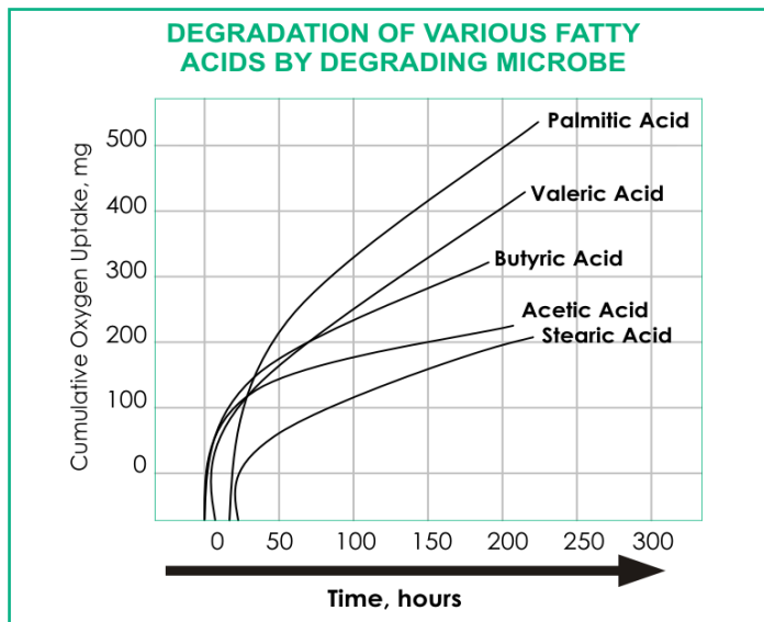
Figure 2: The chart illustrates the degradation performance of the fatty acid degrading strain on several problematic fatty acids as measured by oxygen uptake. The data demonstrates the ability of fatty acid degrader to grow on any one of these compounds as its only source of food. This is especially important with stearic and palmitic acids which can make up as much as 80% of problem grease deposits.
