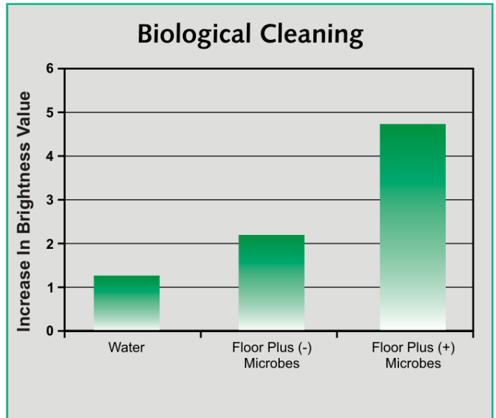
Figure 4: Reflectance data demonstrates the biological removal of grease from floor tiles. Brightness was measured before and after treatment of greasy tiles with a spectrophotometer. An increase in brightness value indicates removal of grease.
